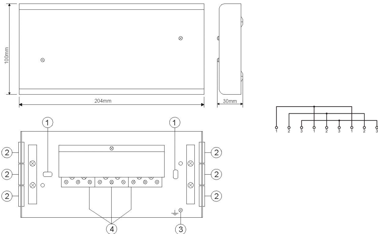
Fig.1. The junction box and wiring diagram.
