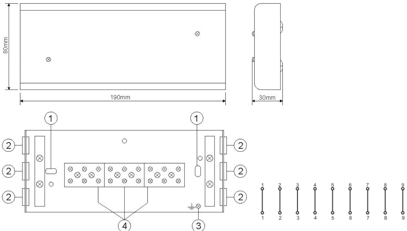
Fig.1. The junction box
