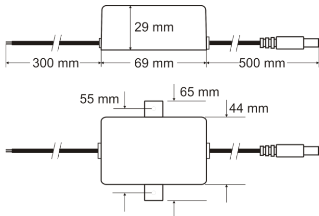
Fig.1. Dimensions of power supply.
